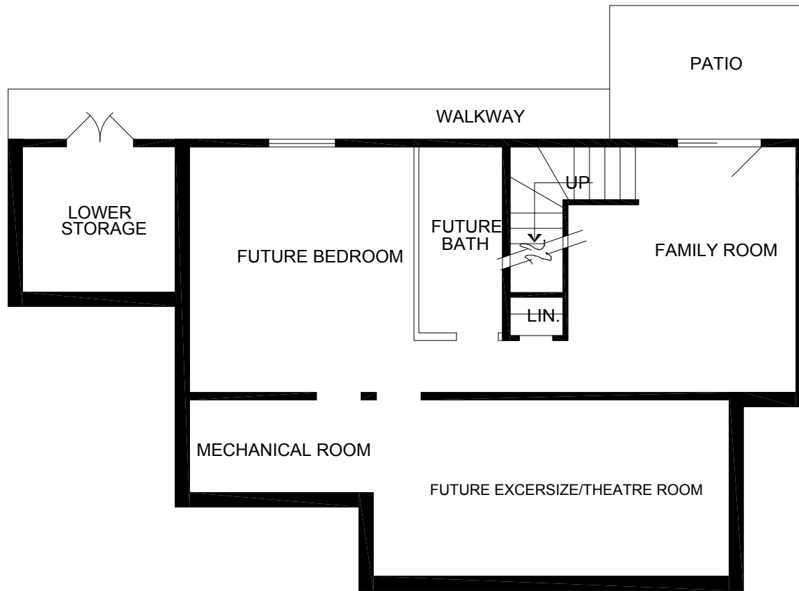
BASEMENT FLOOR AREA = 1,027 SQ. FT. BASEMENT DIMENSION PLAN VIEW
