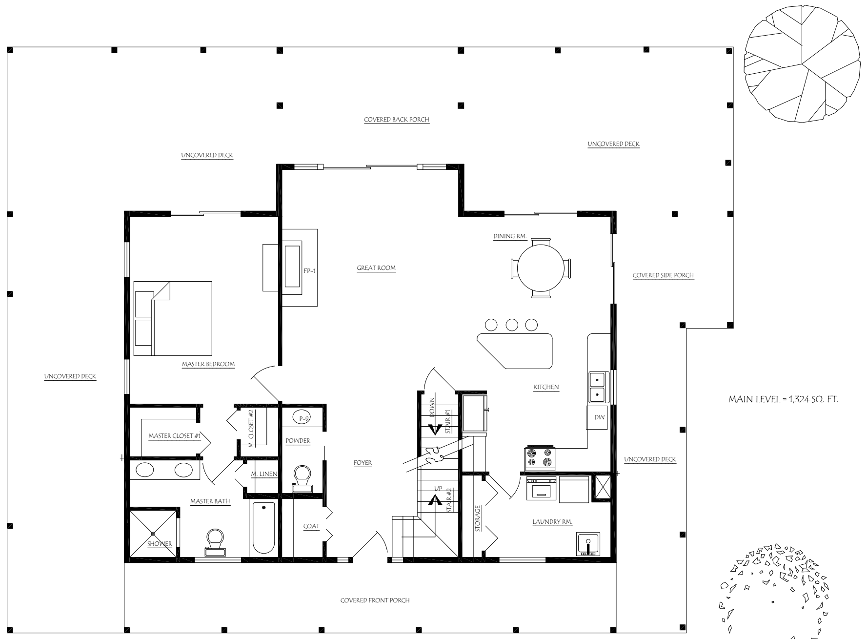
MAIN LEVEL FLOOR PLAN VIEW
